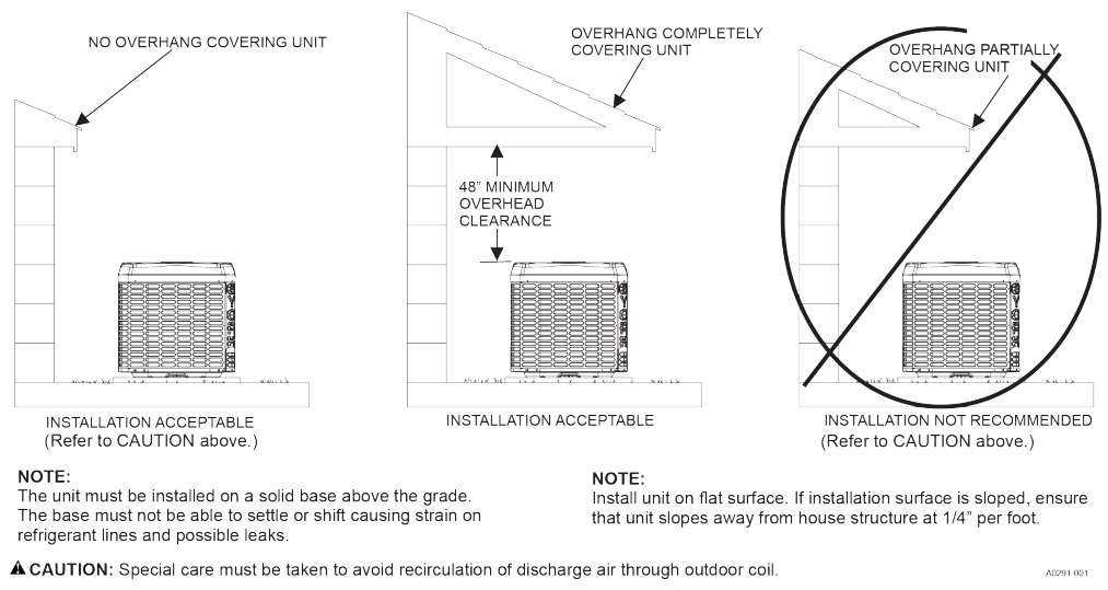
Figure 4: Typical installation
